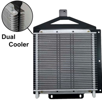
1 x Dual Cooler Bracket with coolers fitted
